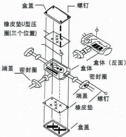
FJH型防爆二通接线盒
